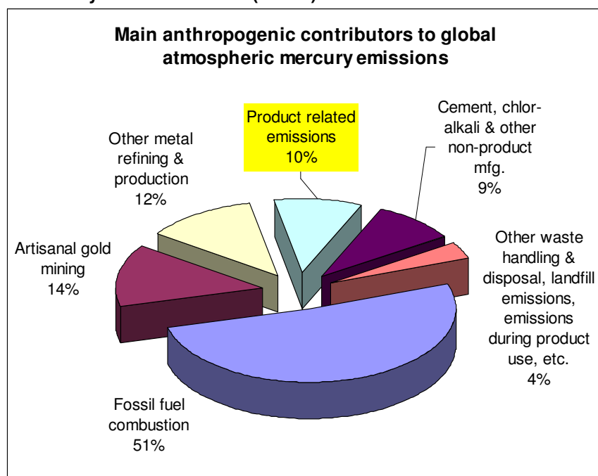
Figure 15 Relative contribution of main anthropogenic sources of mercury emissions to air (~2005)
